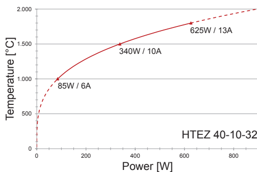
Power vs temperature diagram of HTEZ 40-10-32
