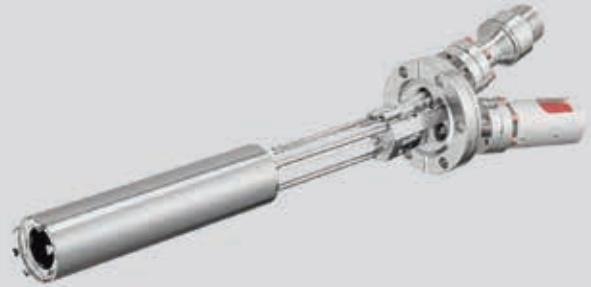
HTEZ 40-10-32 on DN40CF (O.D. 2.75") flange
